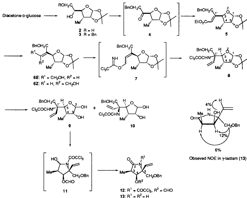
Scheme 1. Bn = -\text{CH}_2\text{Ph} .
